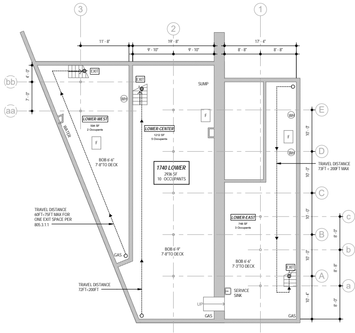
1 LIFE SAFETY PLAN - LOWER LEVEL A01 | 1/8" = 1'-0"
