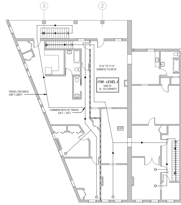
3 LIFE SAFETY PLAN - LEVEL 2 A01 | 1/8" = 1'-0"
