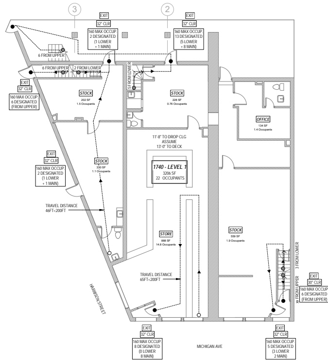
2 LIFE SAFETY PLAN - LEVEL 1 A01 | 1/8" = 1'-0"
