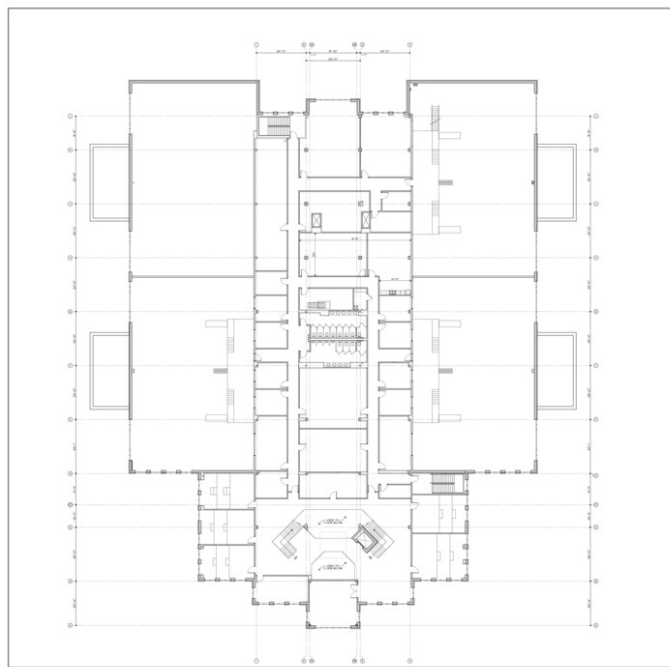
Second Floor Renovation Plan
