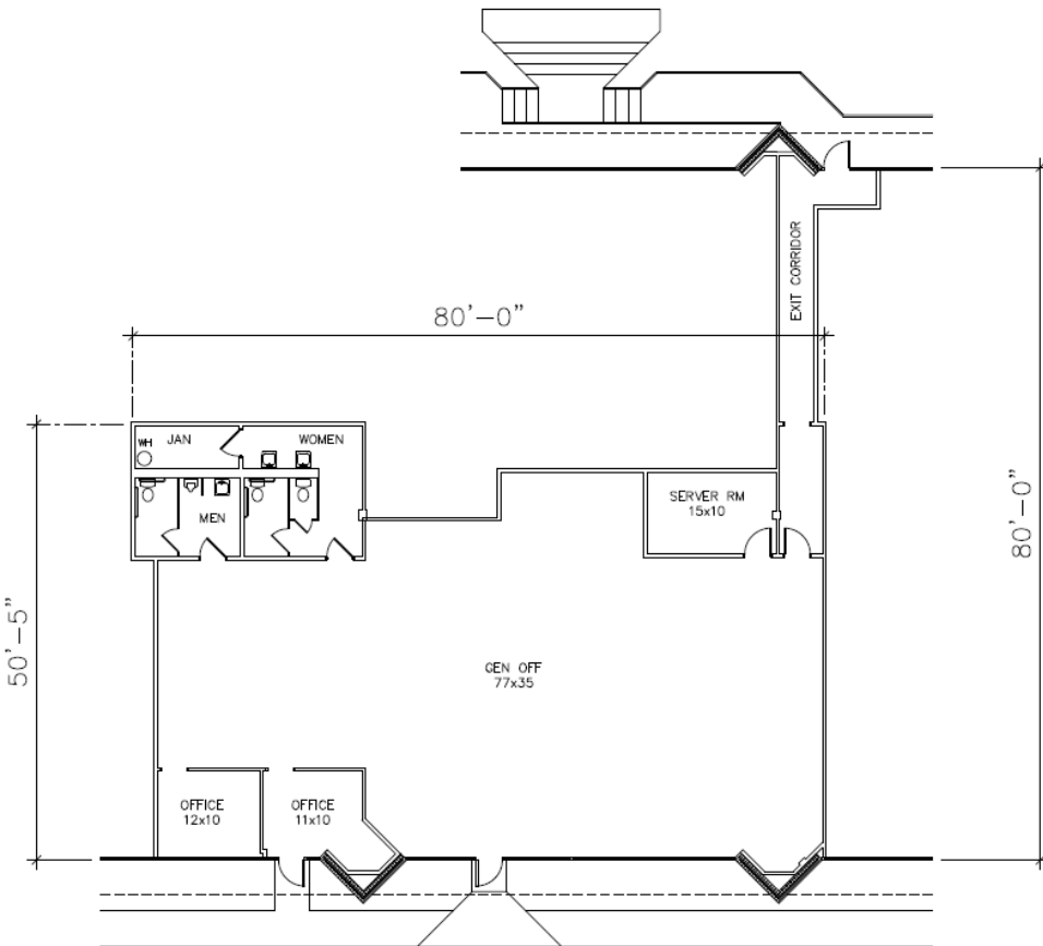
FLOOR PLAN
