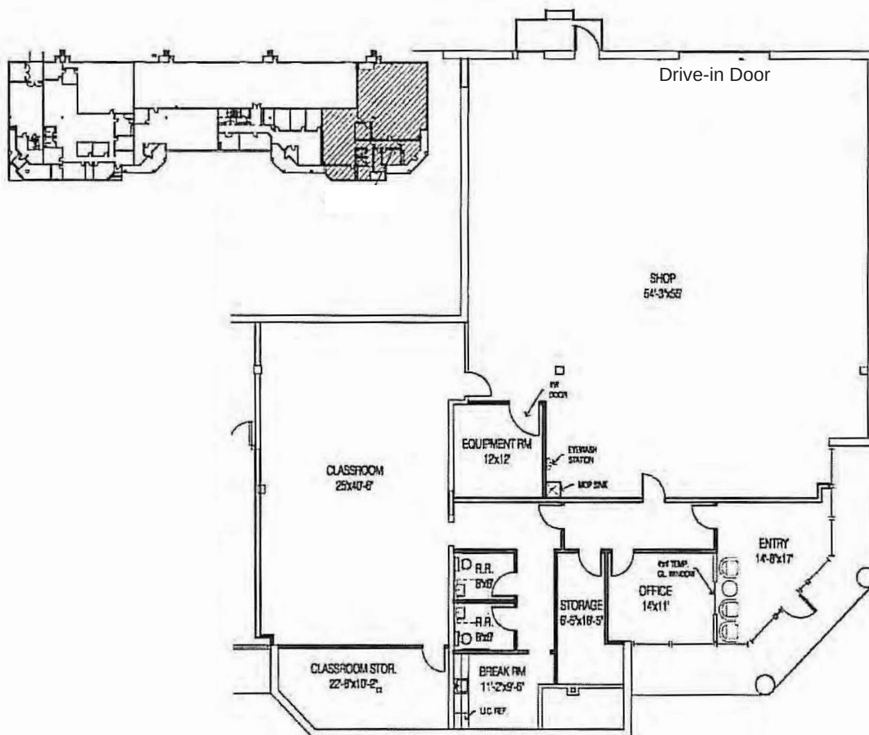
3729 Floor Plan
