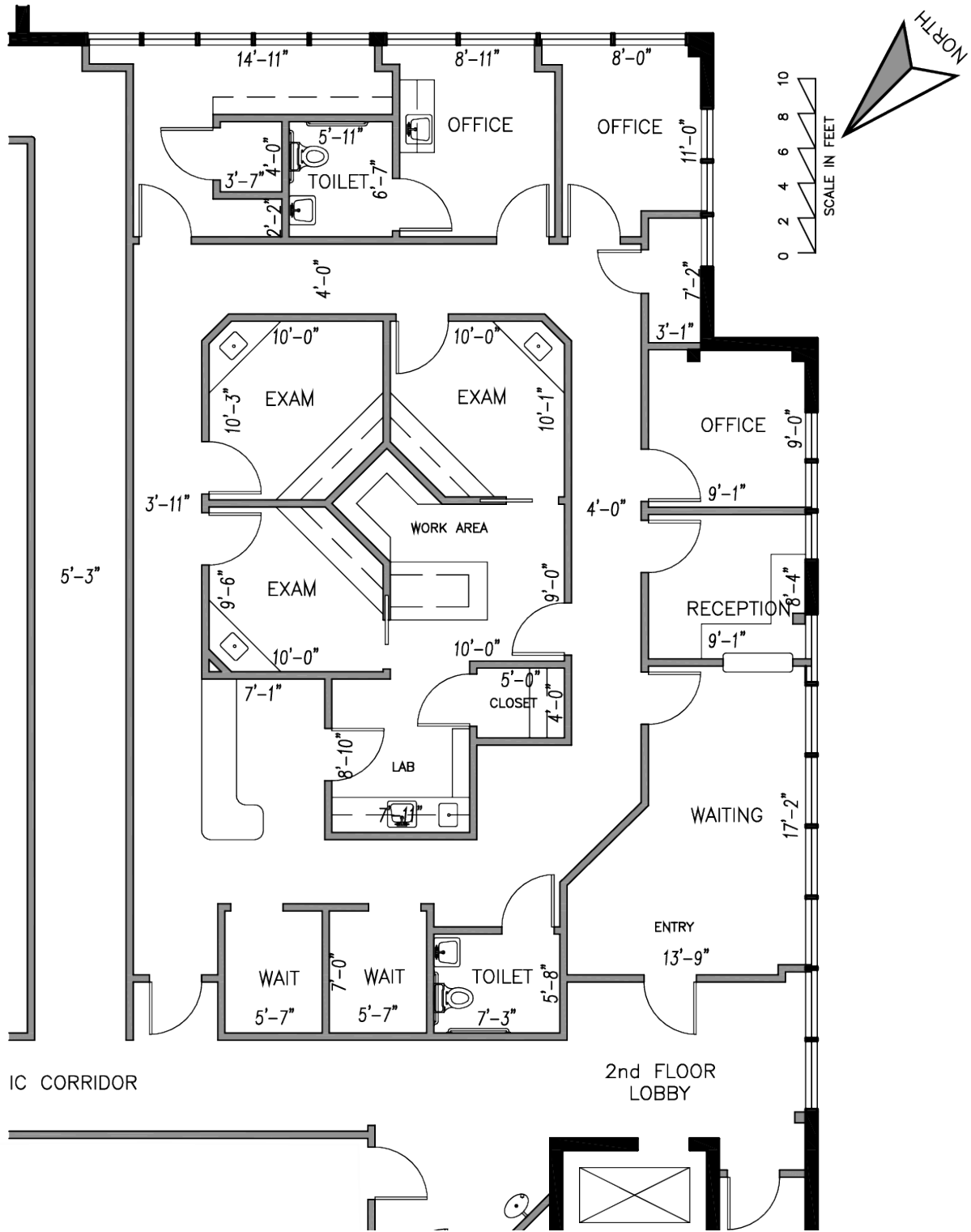
1 AS-BUILT 2,419 SF MEDICAL LAYOUT
