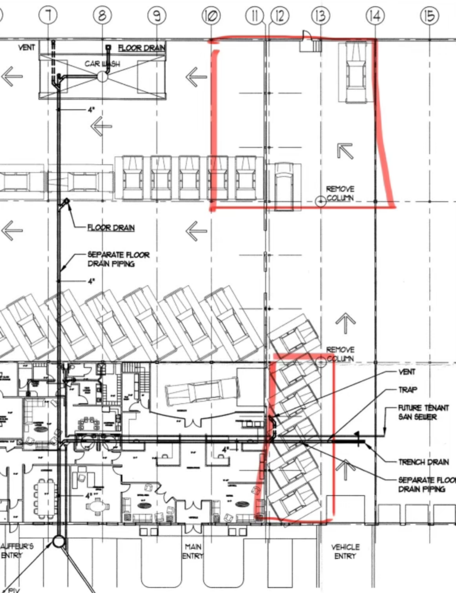
FLOOR PLAN SCALE: 1/16" = 1'-0"
