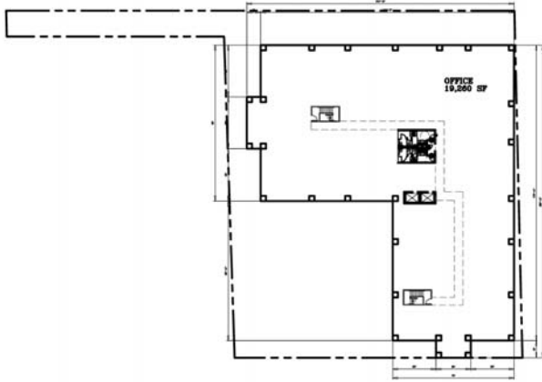
FLOOR 2-5 PLAN 19,200 SF
