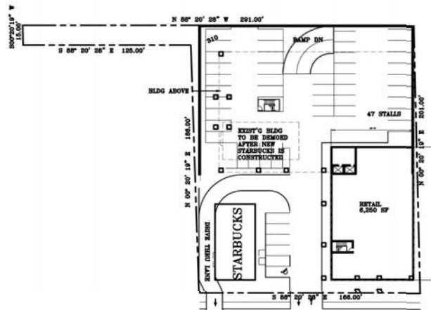
NORTHGATE WAY SITE PLAN
