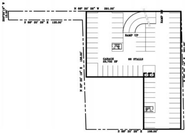
NORTHGATE WAY LEVEL A-B PLAN 23,732 SF
