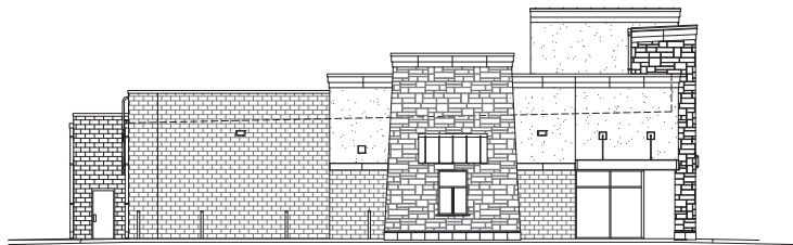
5 SIDE ELEVATION (EAST) 1/8" = 1'-0"
