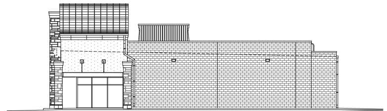
2 SIDE ELEVATION (WEST) 1/8" = 1'-0"
