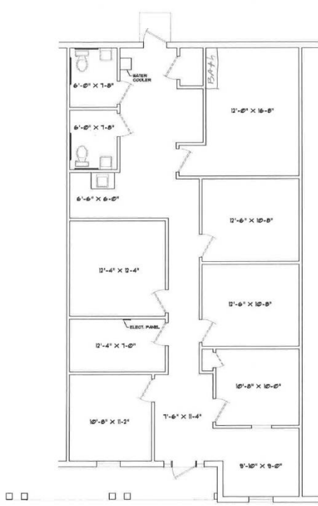
FLOOR PLAN OVERLOOK @ ARKWRIGHT SCALE: 1/8" = 1'-0" 1/20 S.F.
