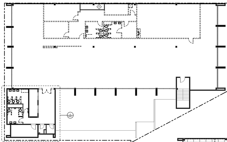
Demolition Plan
