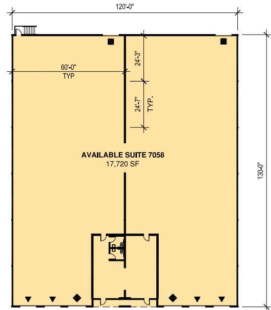
FIRST FLOOR PLAN Scale: 0' 6" 12" 18" 30"
