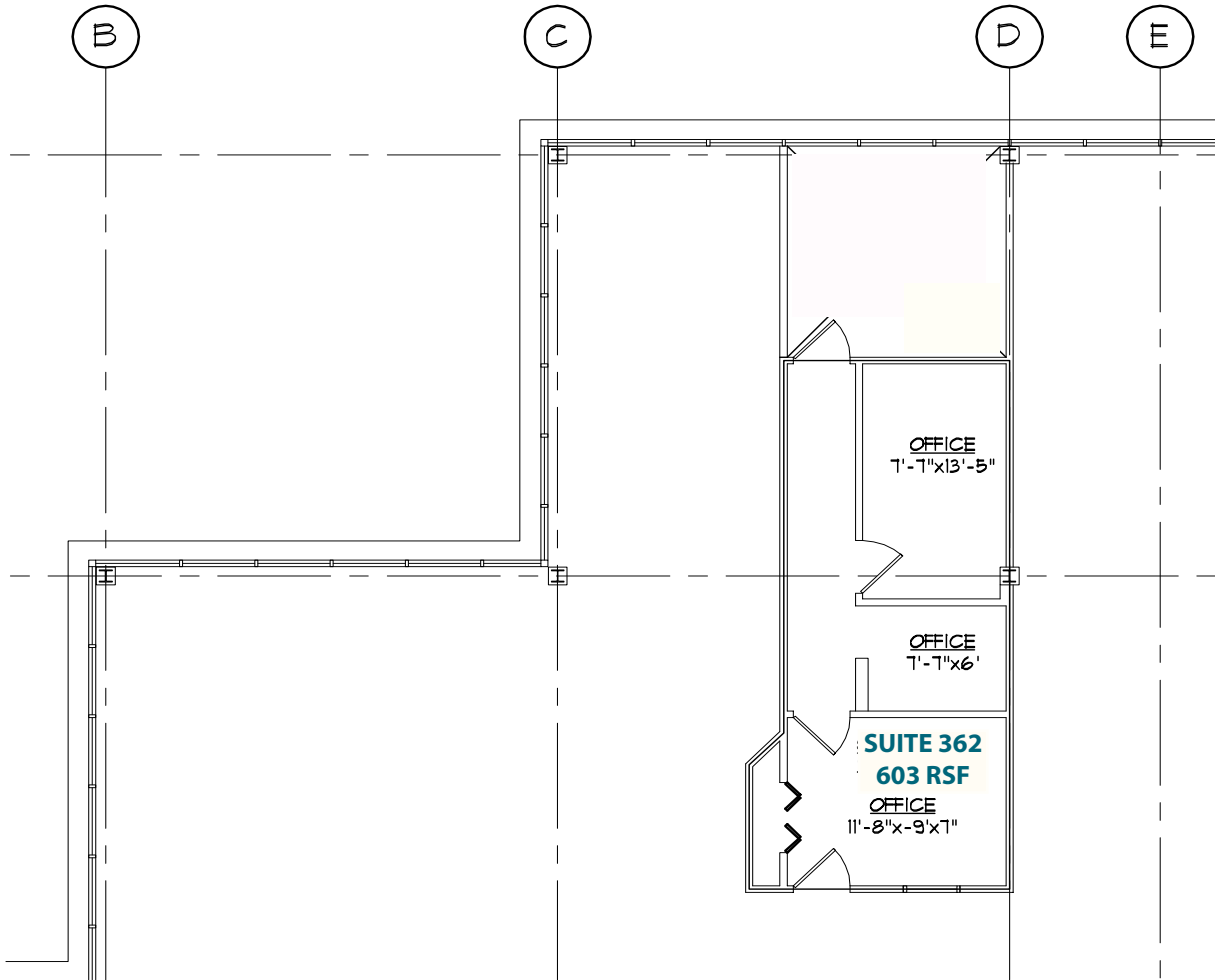
1 THIRD FLOOR PLAN L-3 | L-3 SCALE: 1/8"=1'-0"
