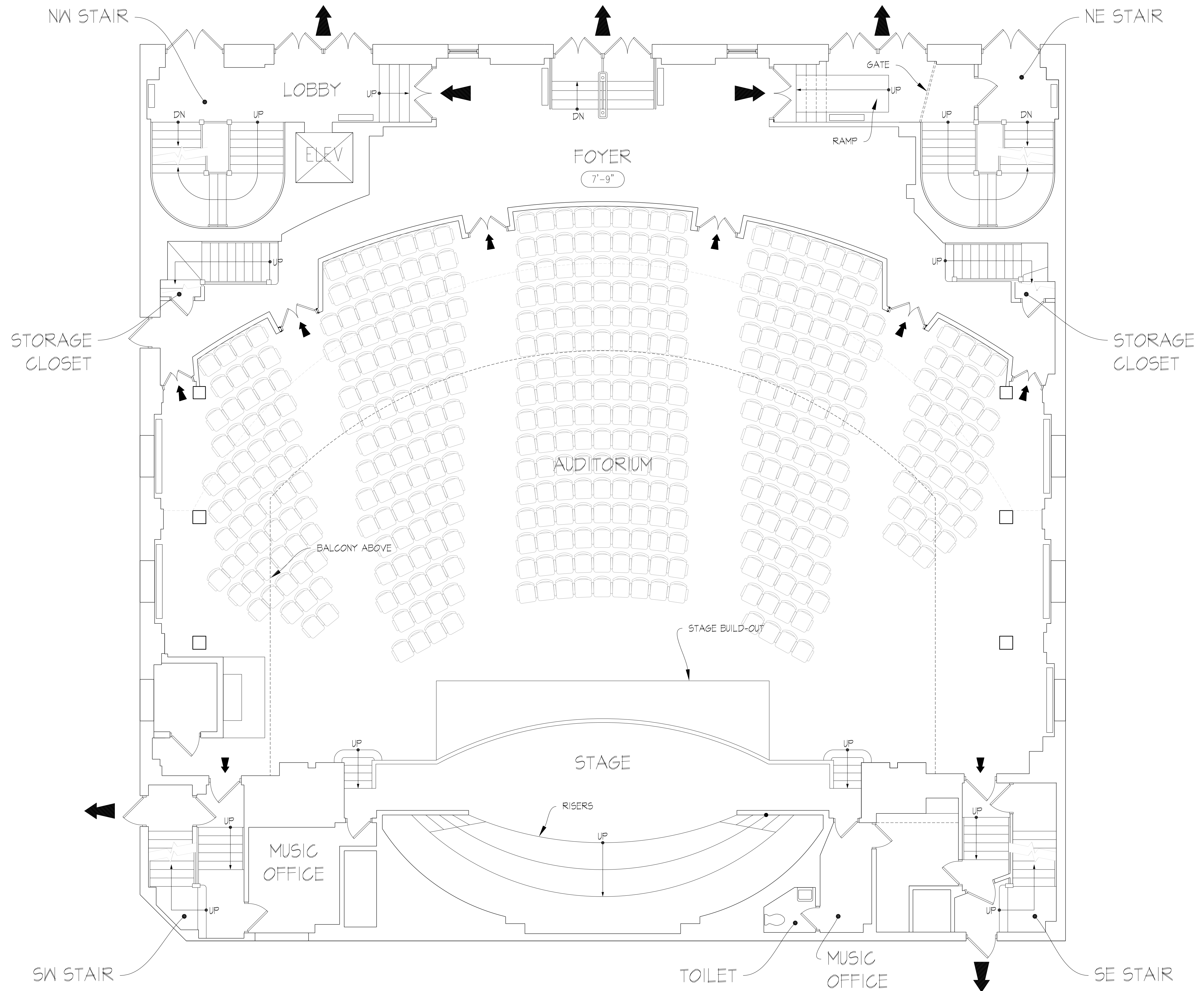
1ST FLOOR EXISTING FLOOR PLAN
