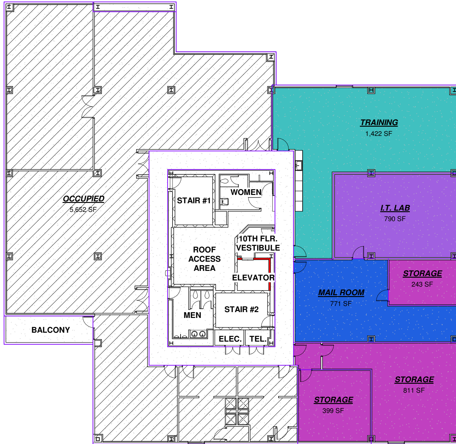
1 10TH FLOOR - EXISTING 1/16" = 1'-0"
