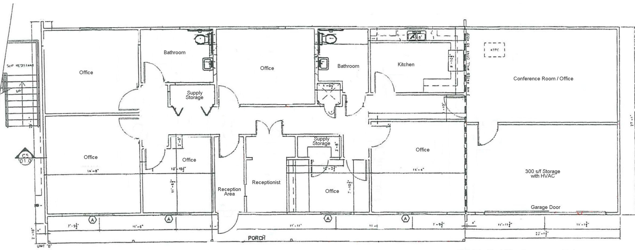
A1 1ST. FLOOR PLAN (UNIT C) NOT TO SCALE
