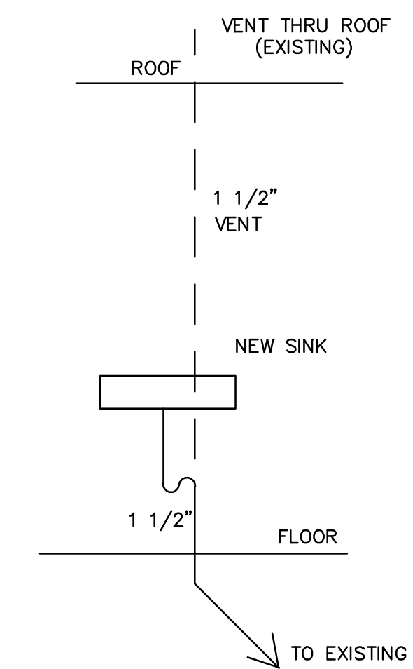
PLUMBING RISER DIAGRAM NO SCALE
