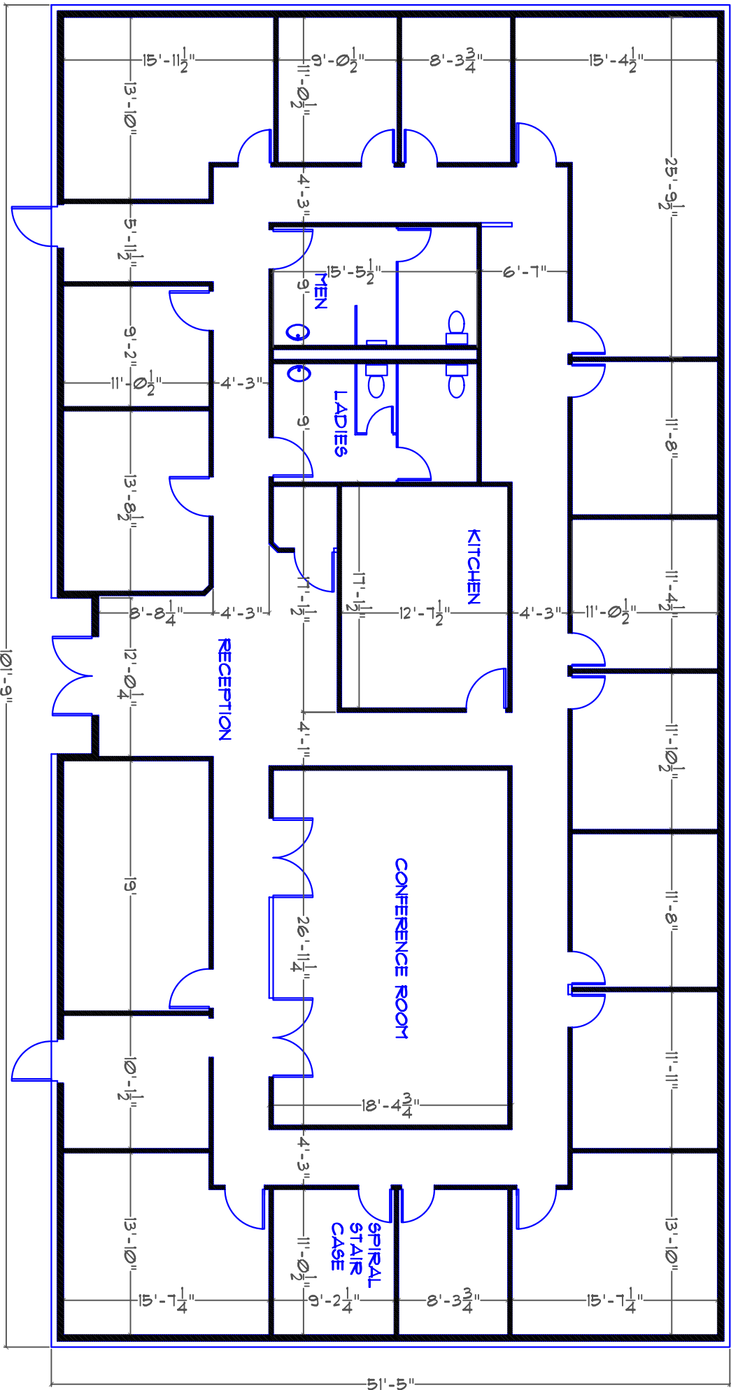
3221 Summit Square Place - Main Floor Plan
