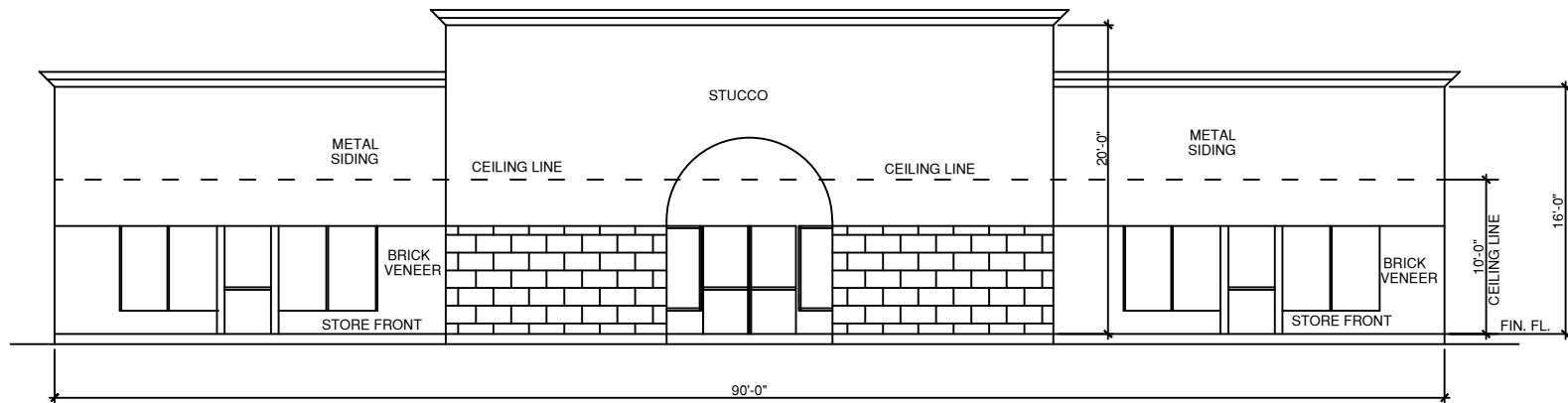
NEW FRONT ELEVATION
