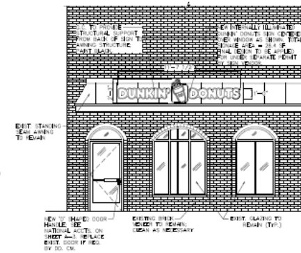
PROPOSED FASCIA SIGN SCALE: 1/2" = 1'-0"
