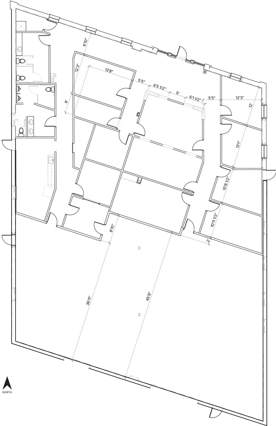
Floor Plan
