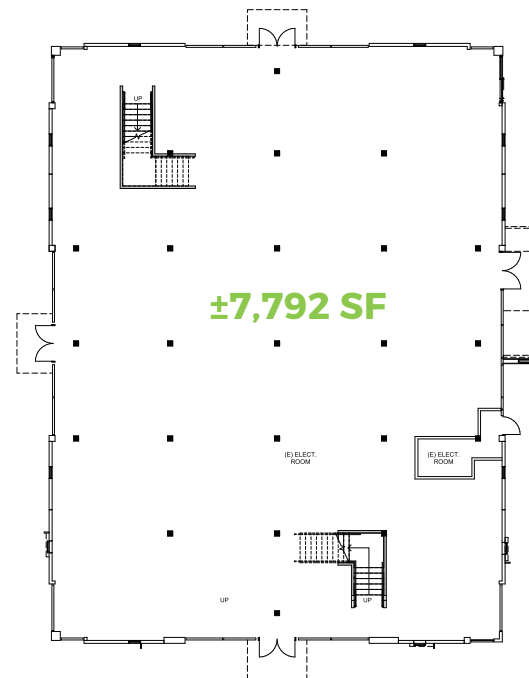
BUILDING A FIRST FLOOR PLAN
