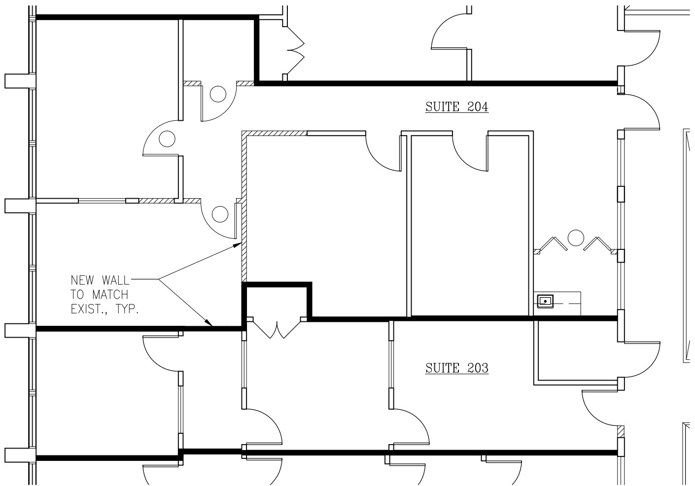
1 SUITES 203 & 204 NEW FLOOR PLAN SCALE: 1/8"=1'-0"
