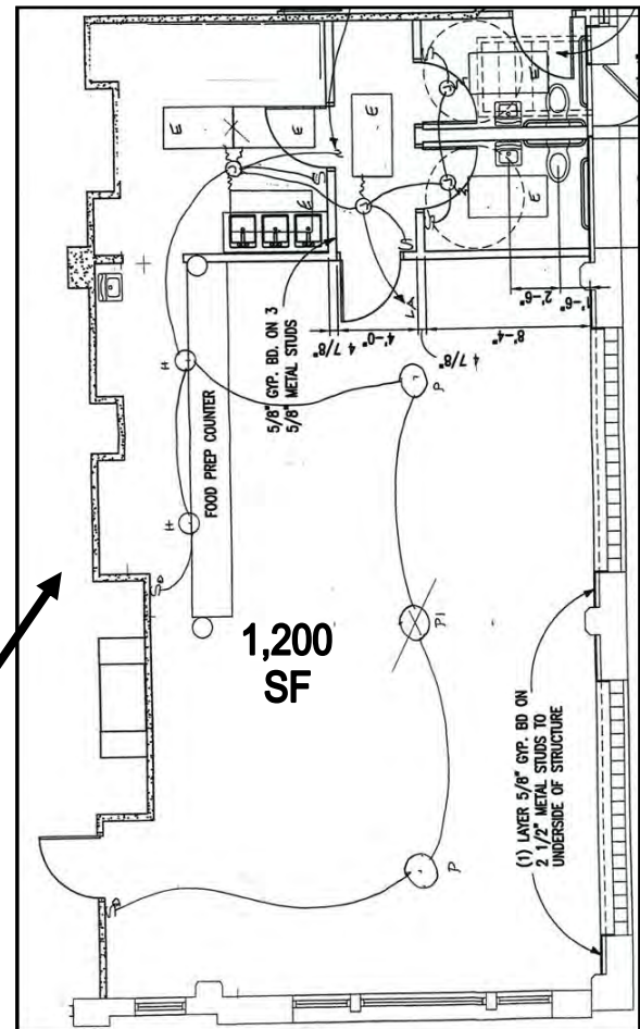
1st Floor - Restaurant Space
