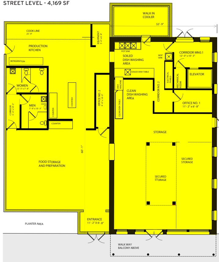
STREET LEVEL - 4,169 SF
