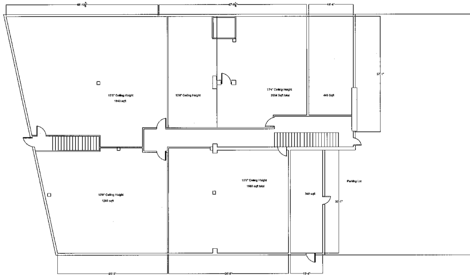
Harwood Floor Plan Level 1 Scale: 3/32" = 1'0"
