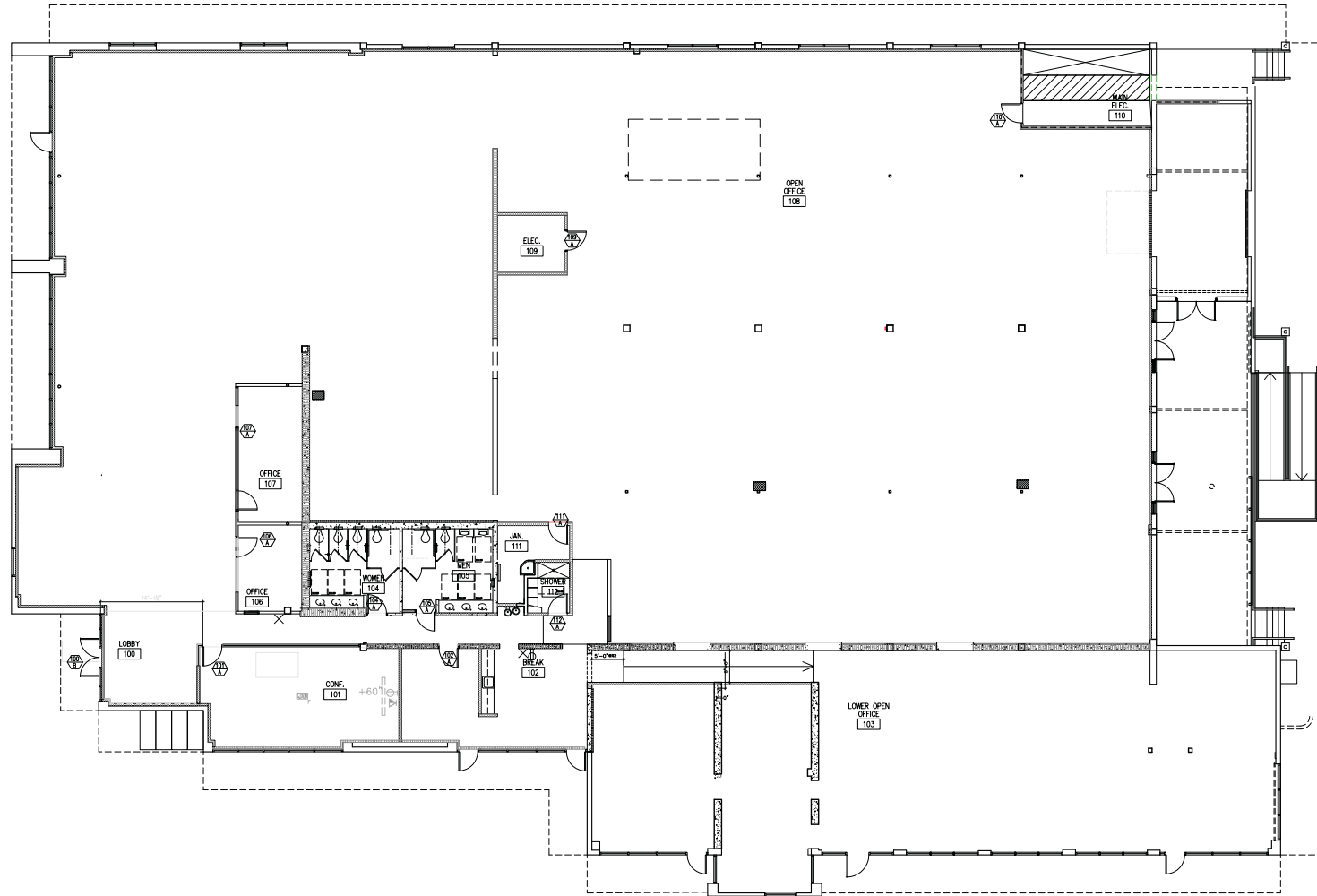
1 PROPOSED FLOOR PLAN A2 SCALE: 1/8" = 1'-0"
