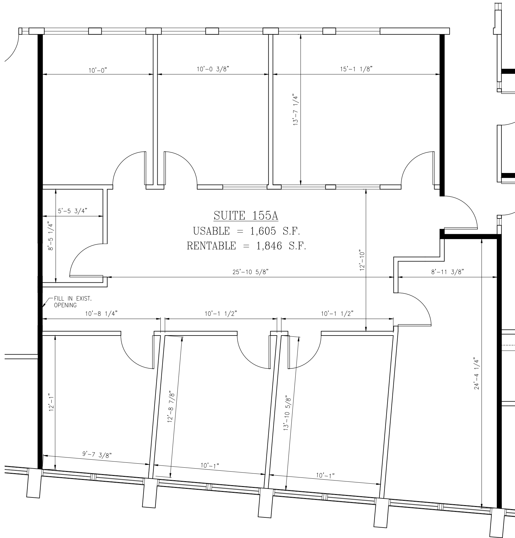
1 DIMENSIONED FLOOR PLAN SCALE: 3/16"=1'-0"
