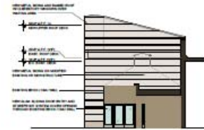
D PARTIAL EAST ELEVATION 1/8" = 1'-0"
