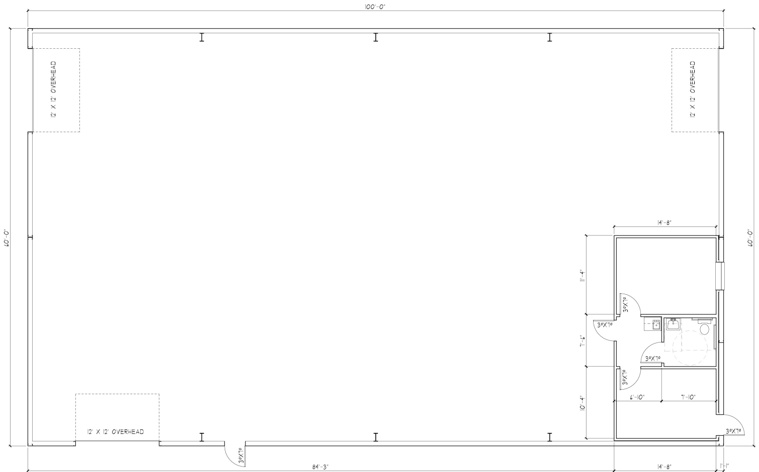
60'X100' FLOOR PLAN
