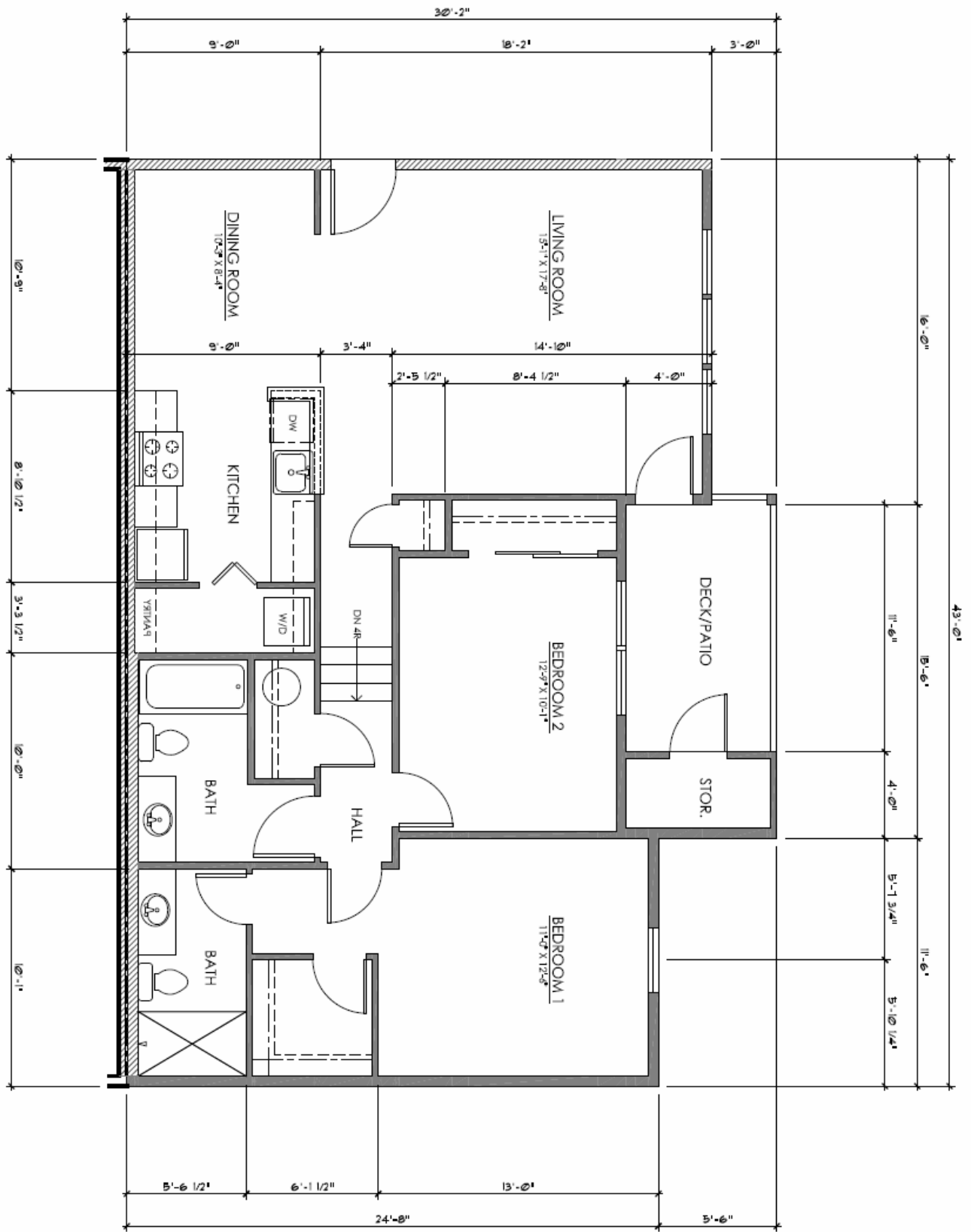
2 UNIT TYPE 2C FLOOR PLAN 1/4" = 1'-0" A32
