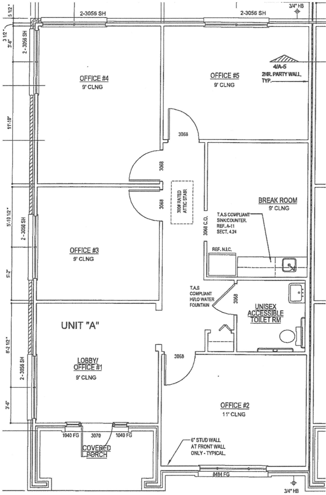
01 Floor Plan 1/4" = 1'-0" 0 1 2 3 4 5 10
