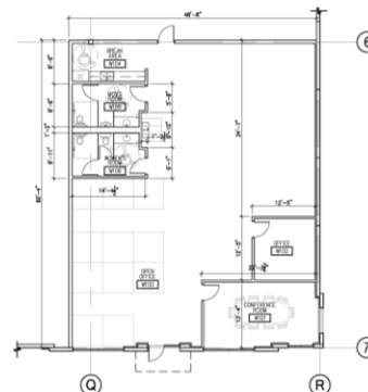
2 ENLARGED OFFICE PLAN SCALE: 1" = 20'-0"
