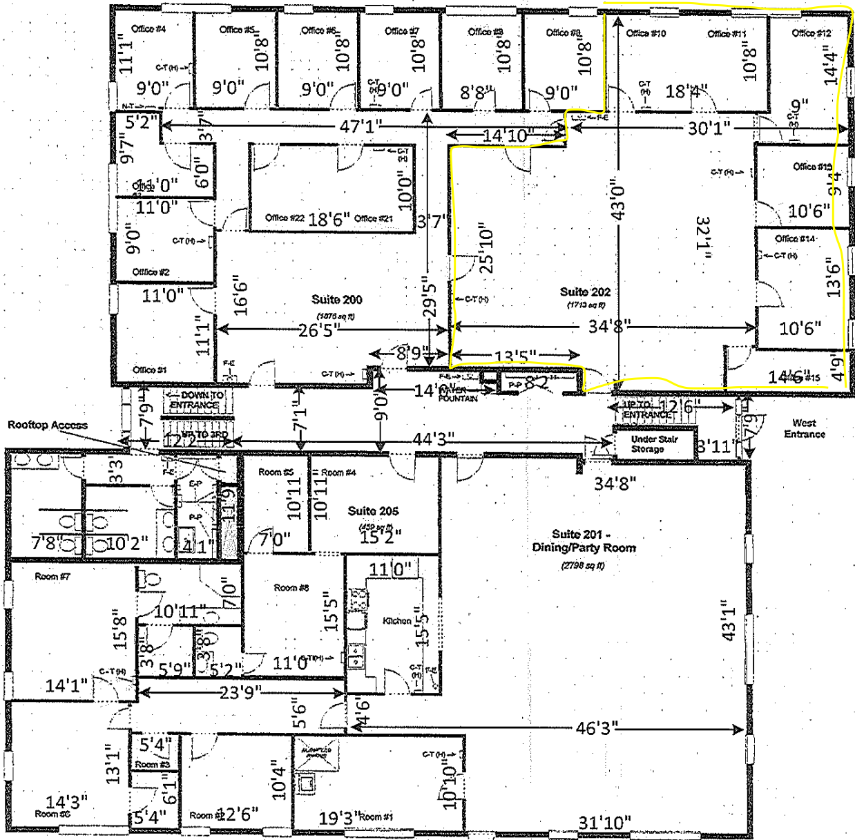
Second Floor - 7340 Sq Ft
