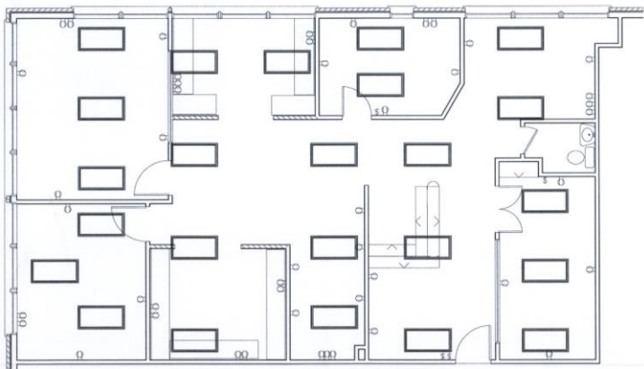
Electrical Plan
