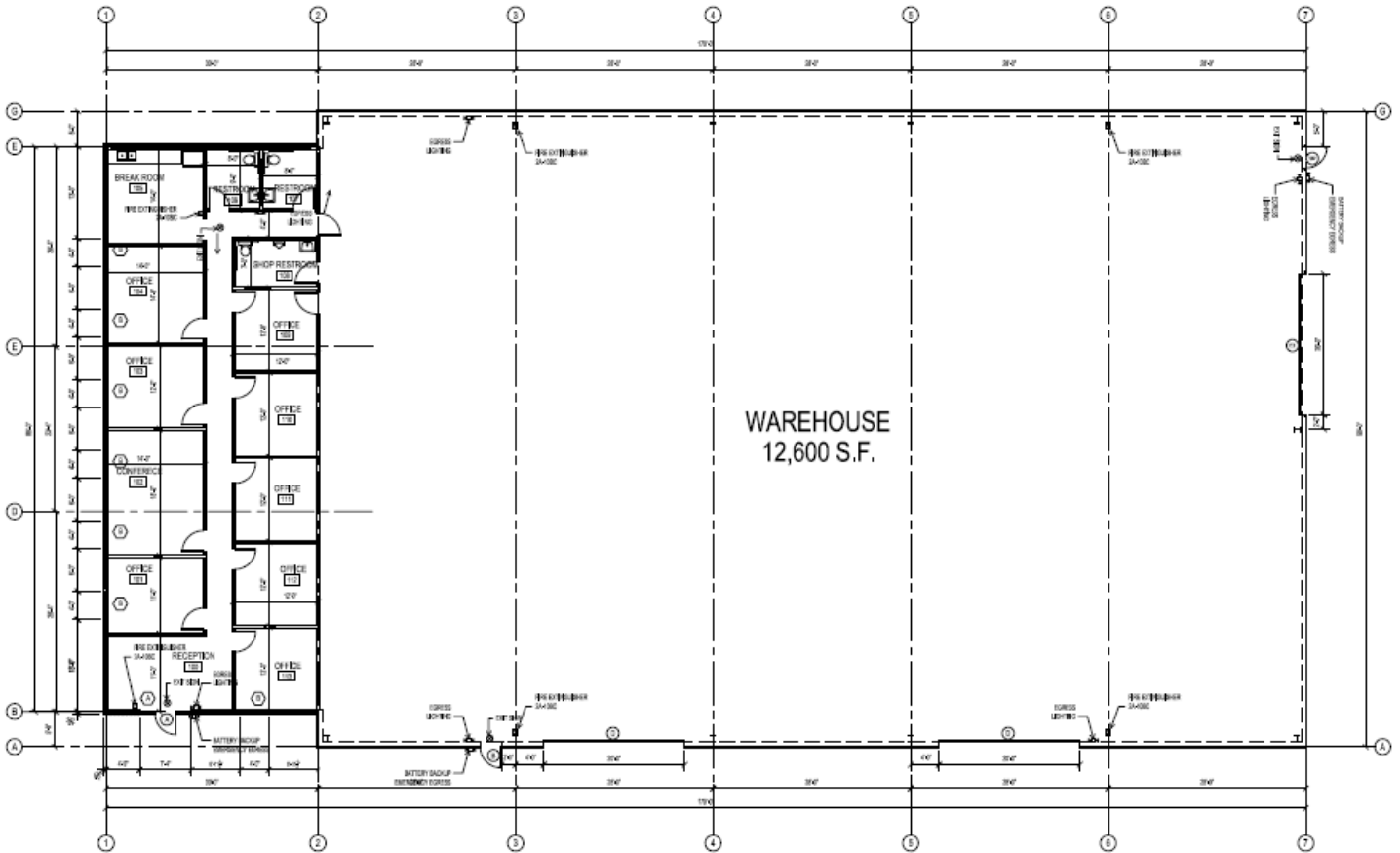
1 1/8"=1'-0" FLOOR PLAN
