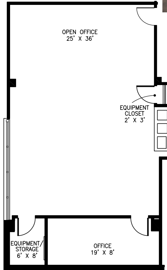
3RD FLOOR KEY PLAN
