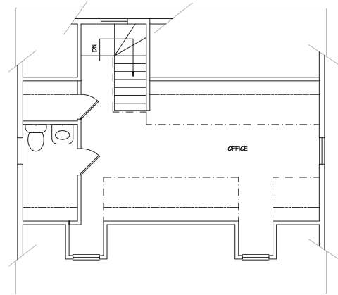
3 ATTIC PLAN 394 SQ. FT. SCALE: 1/4" = 1'-0"
