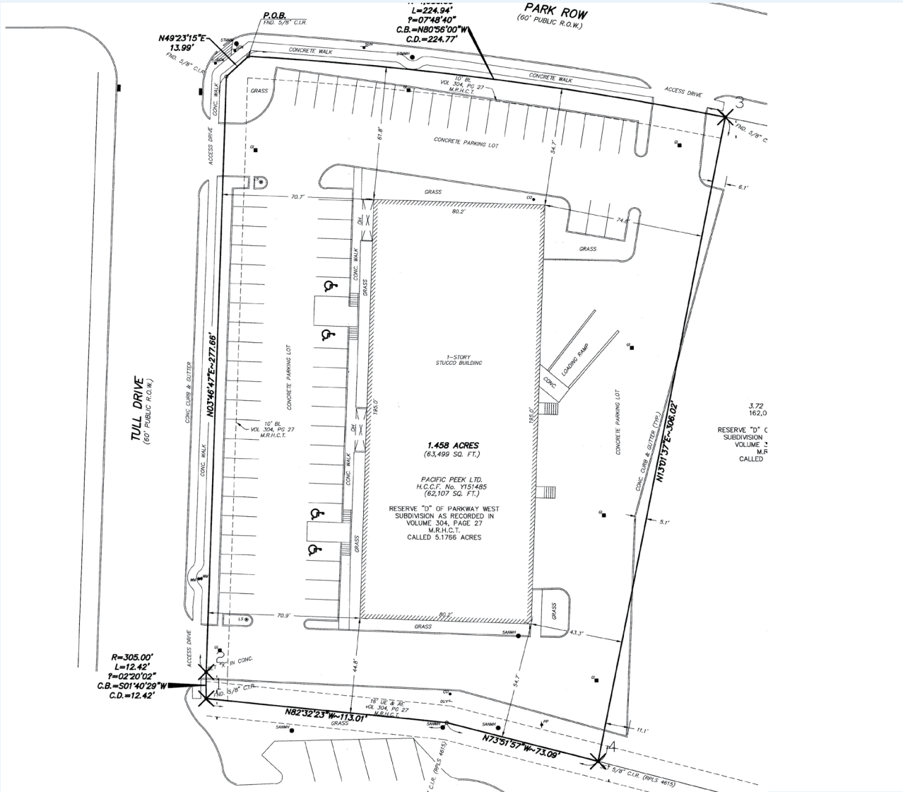
PROPERTY SURVEY
