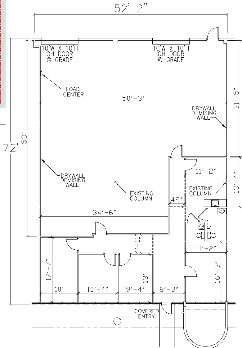
SPACE PLAN
