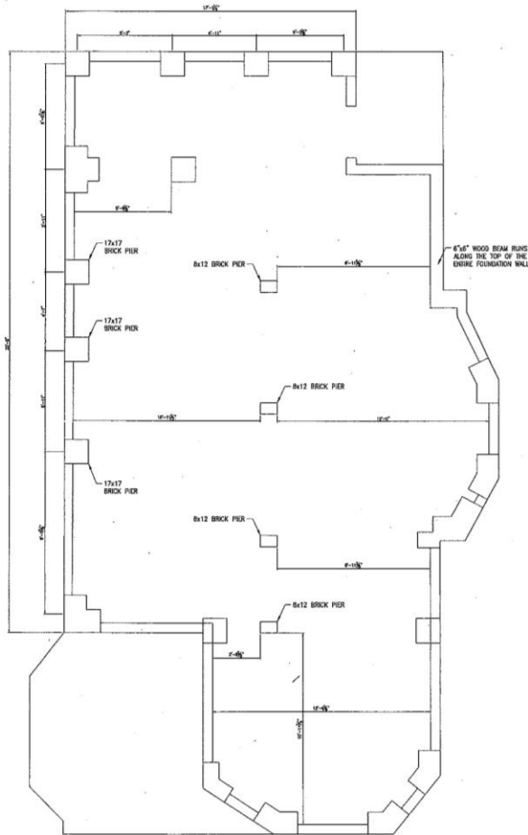
PLAN VIEW- CRAWL SPACE 38' x 1'-0"
