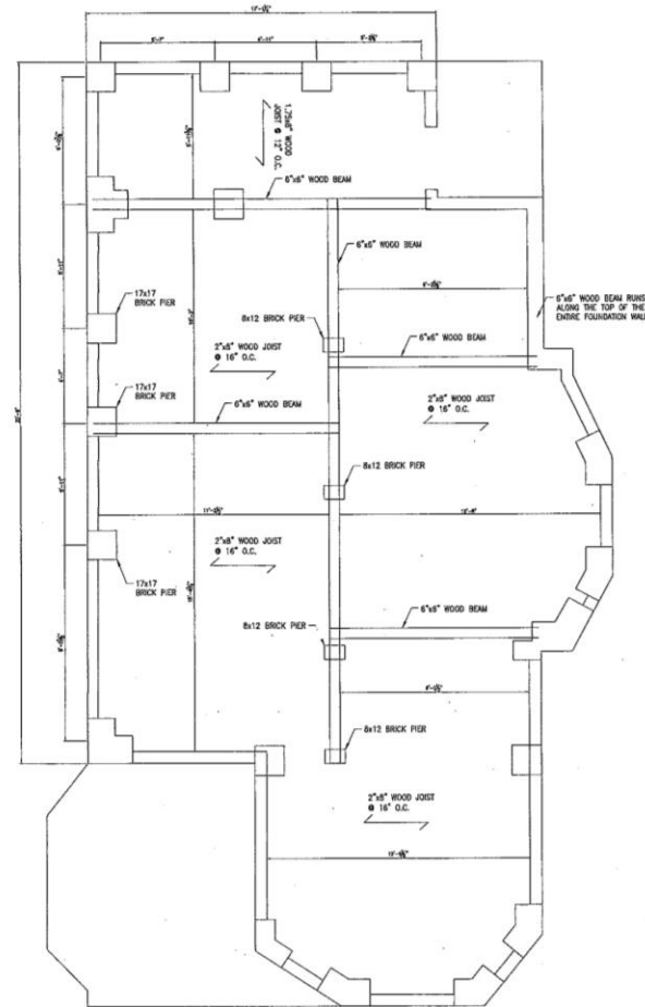
PLAN VIEW- FIRST FLOOR FRAMING 38' x 1'-0"
