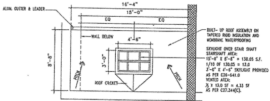
6 STAIR - "B" BULKHEAD PLAN SCALE: 1/4"=1'-0"
