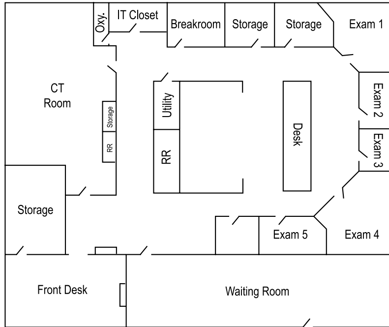
First Choice ER - Floor Plan Unite A (4,000 SF)
