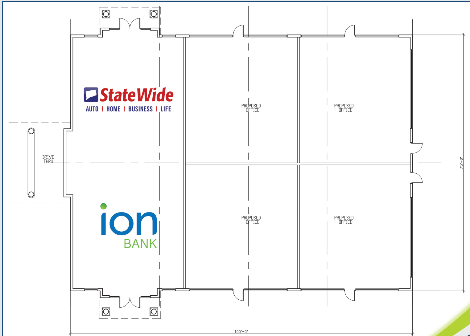
A FLOOR PLAN A-1 1/8"=1'-0"
