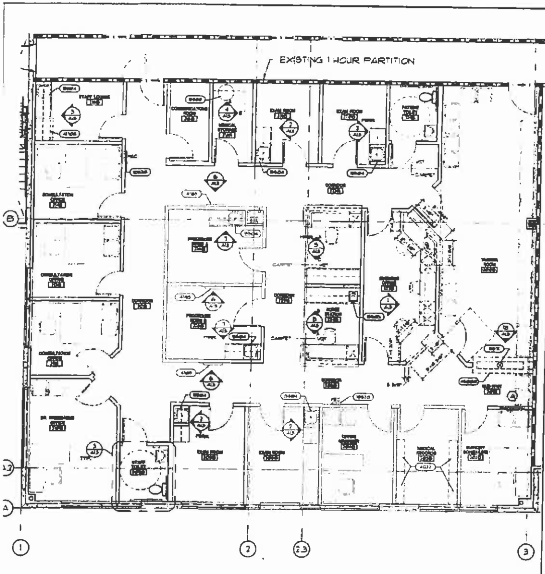
EQUIPMENT PLAN SCALE: 1/4" = 1'-0"
