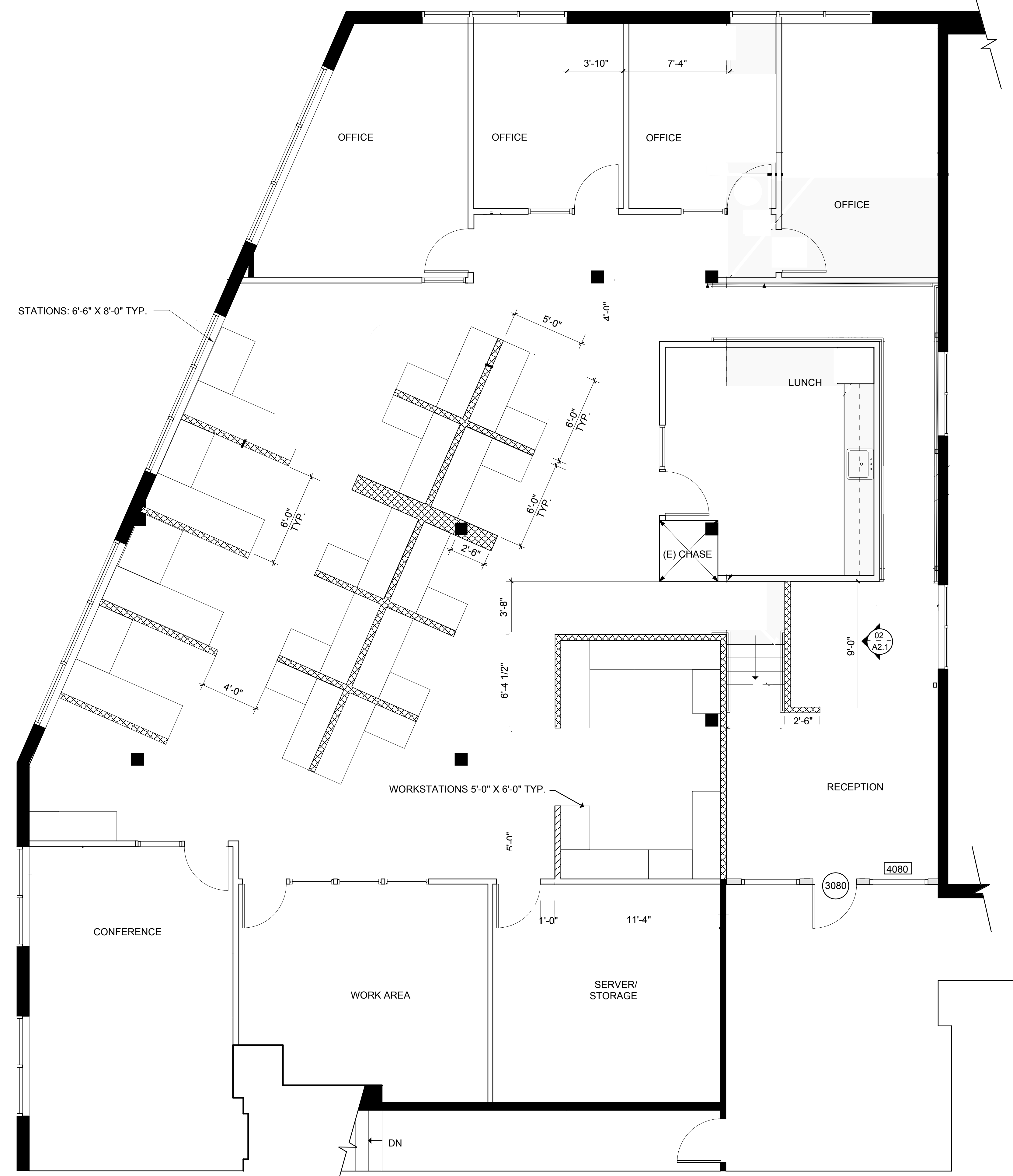
01. Floor Plan
