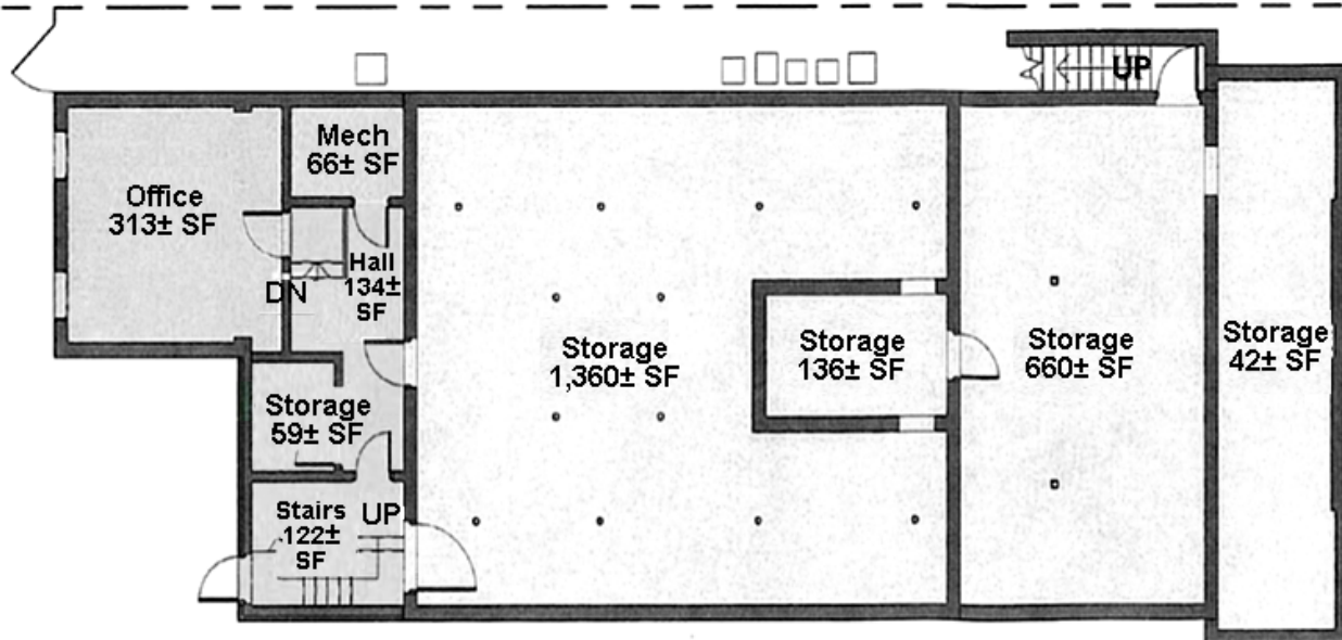
LOWER LEVEL
