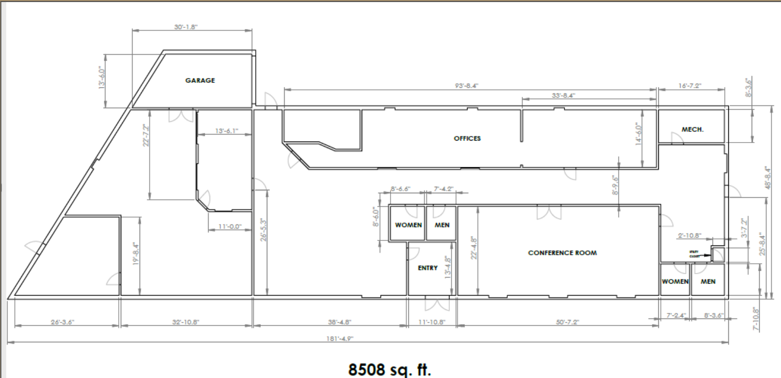
Building B: Floor Plan
