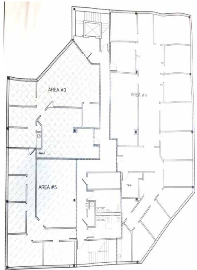
FLOOR PLAN - SECOND FLOOR
