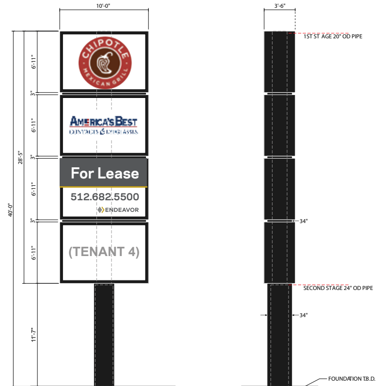
A D/F MULTI-TENANT PYLON SIGN SCALE: 3/16"=1'-0" (1) RE QUIRED
