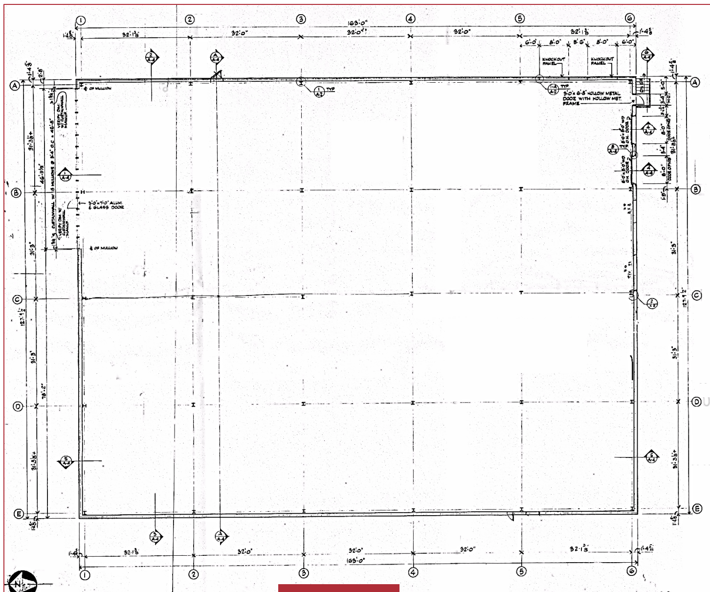
Floor Plan
